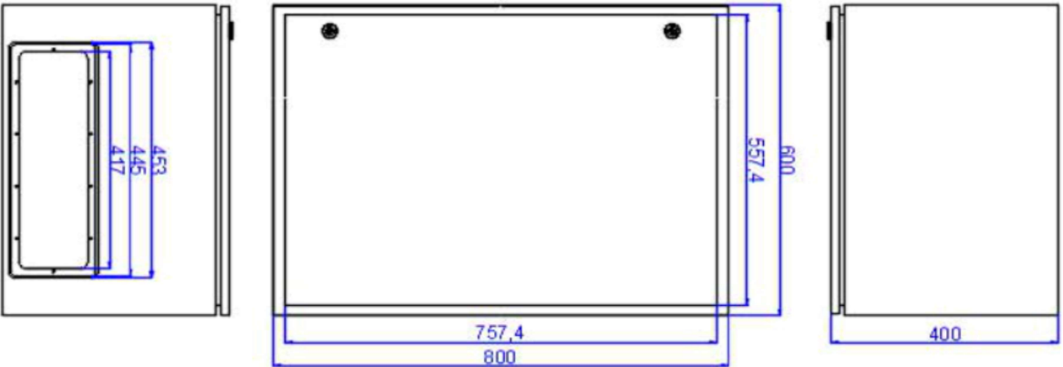
EKM806040 | 800H 600W 400D, IP66 Electrical Enclosure
